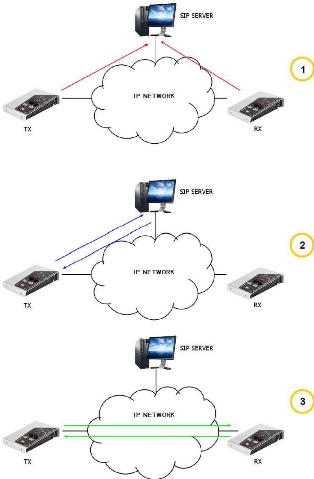
SIP protocol operation diagram. Phase 1: Registration. Phase 2: Search for the called device in the SIP server database. Phase 3: Establishment of the connection
