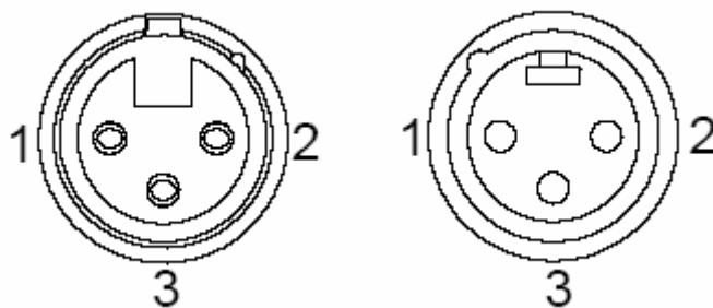
Input - Female
