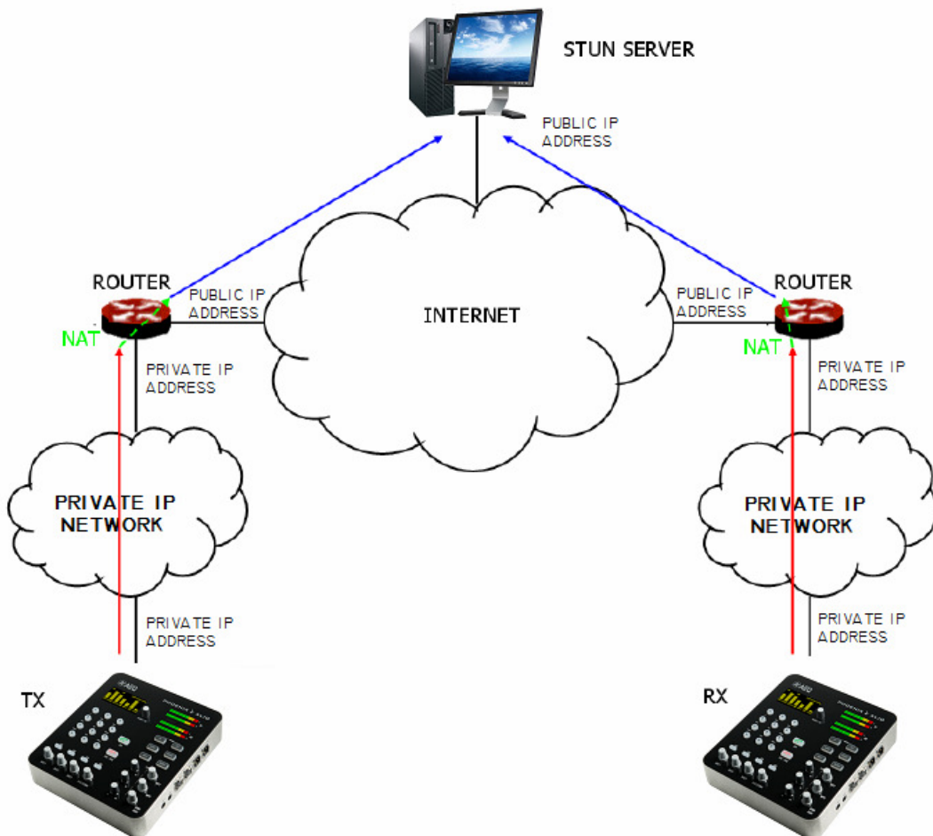
Registration in a STUN server
