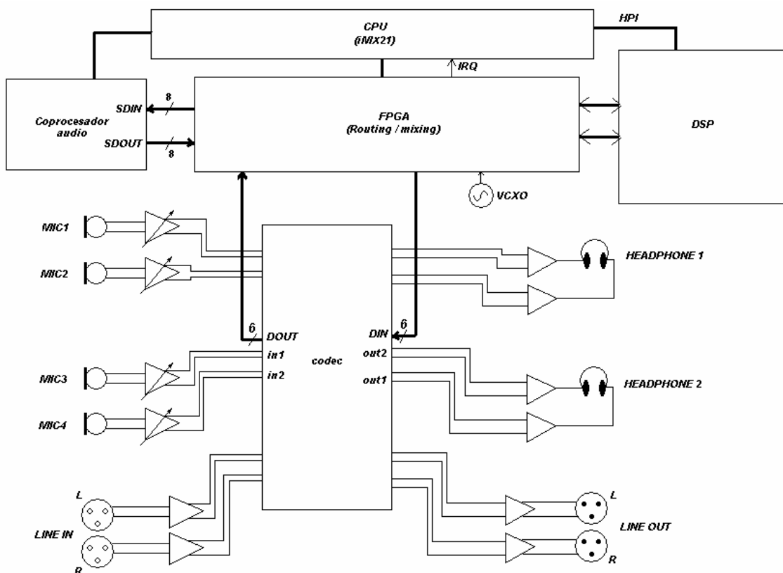
Audio inputs/outputs structure
